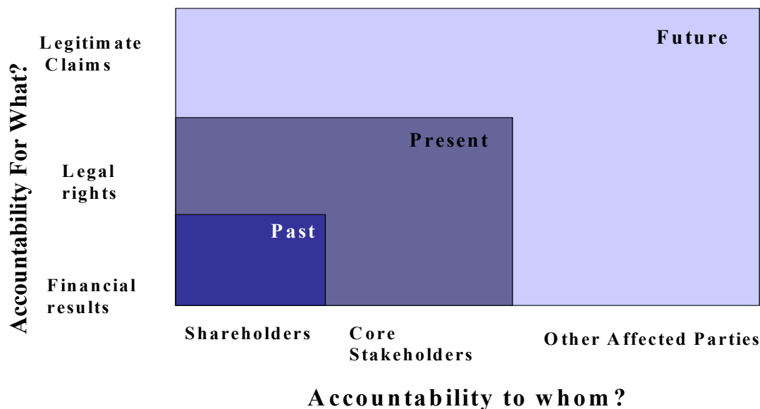
Figure 3: Accountability Shifts
